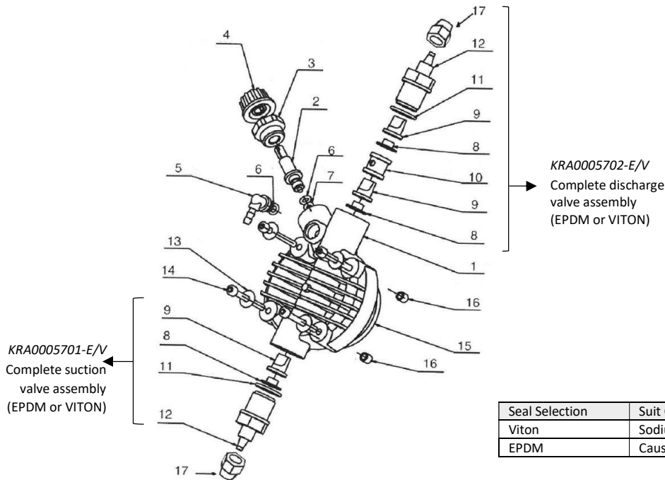
Complete Pump Head SCP0003002 (Viton) SCP0003006 (EPDM)
